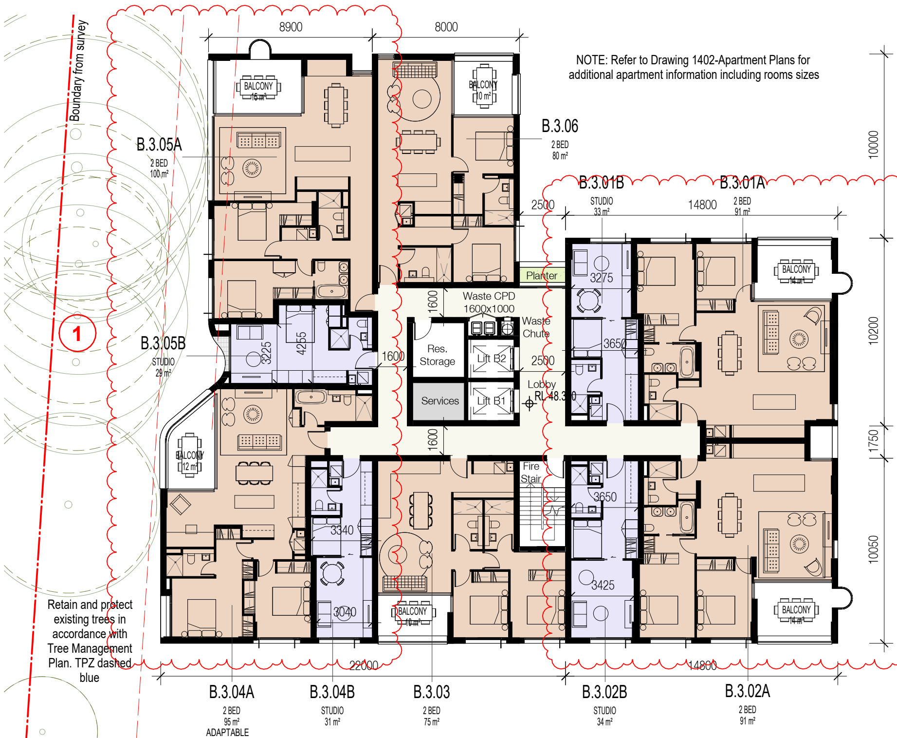
B-Level 3 1: 200@A1
