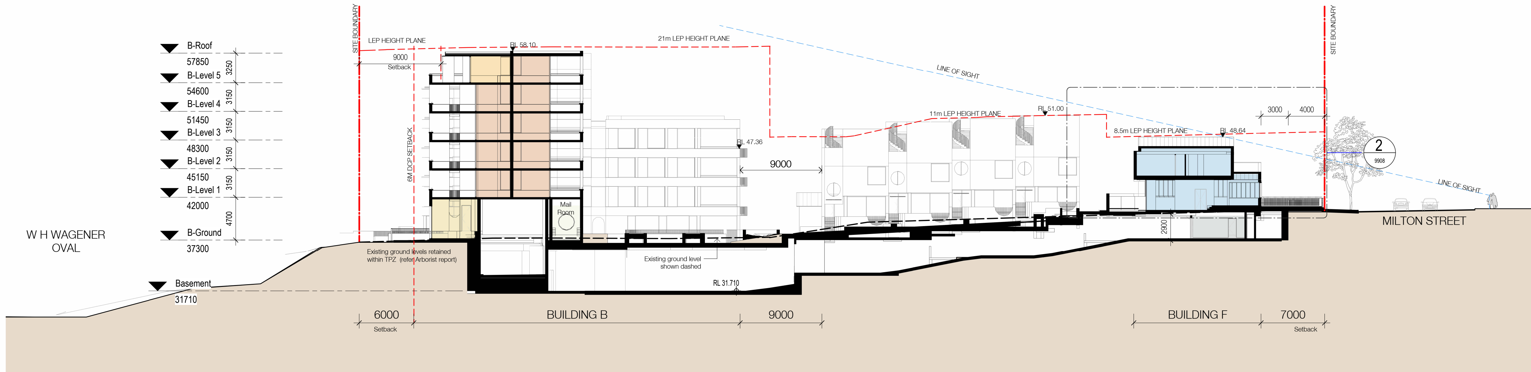
Section B 1:250@A1
