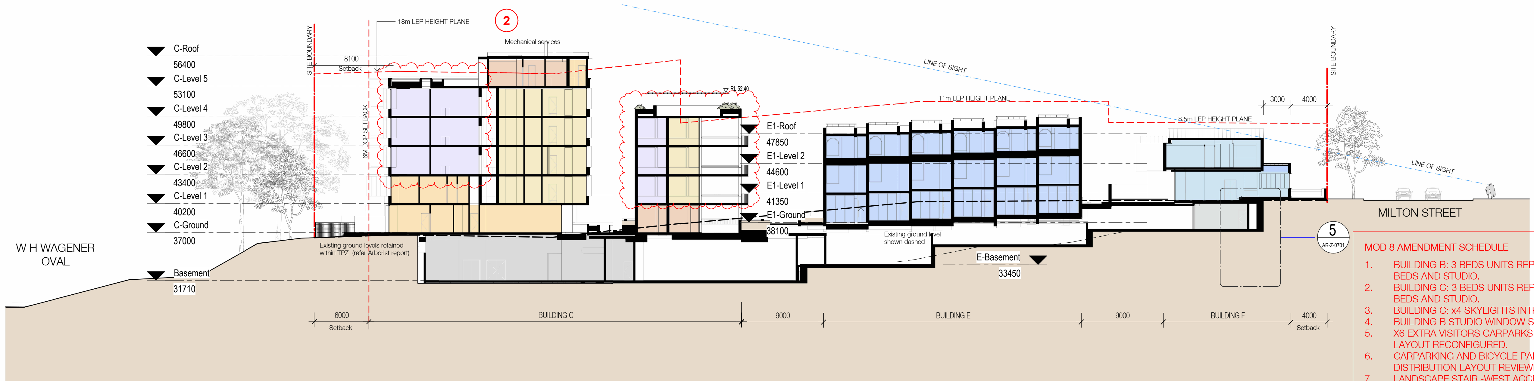
Section C 1:250@A1
