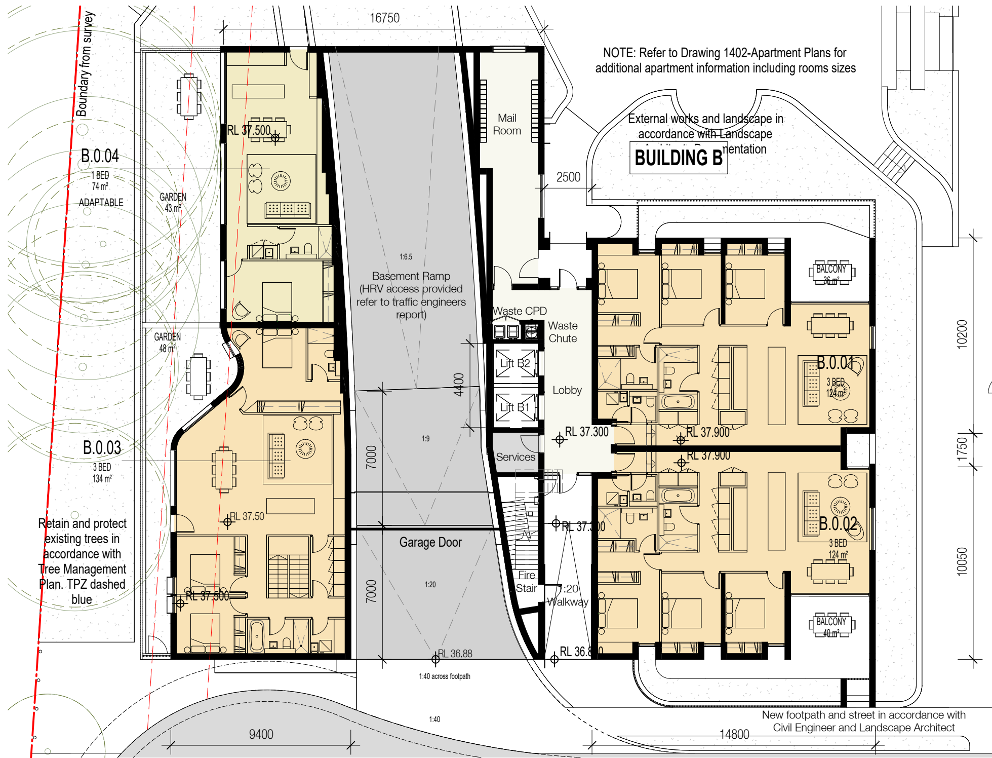
B-Ground 1: 200@A1
