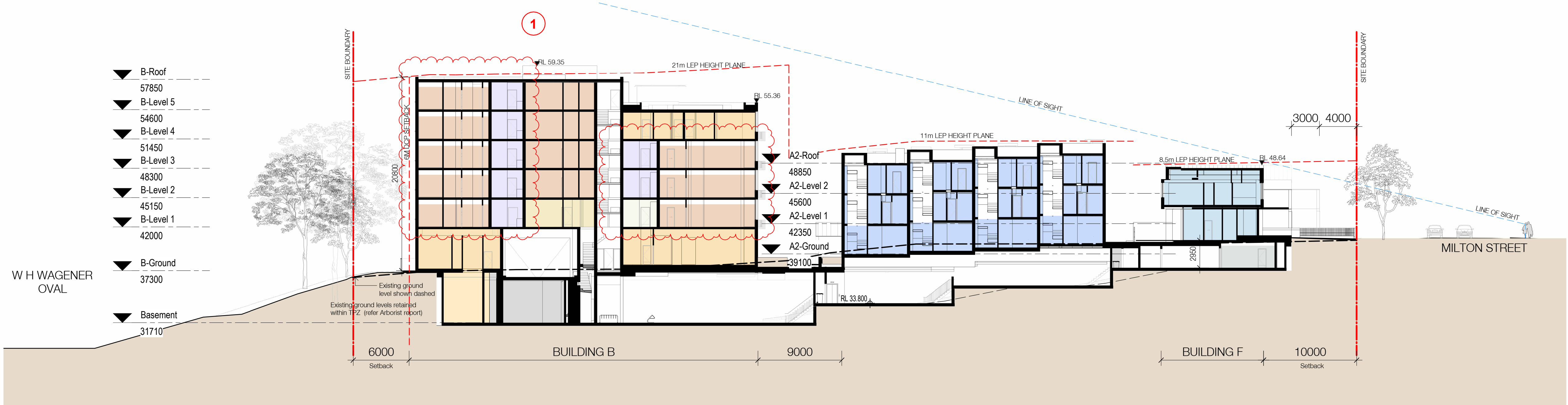
Section A 1:250@A1
