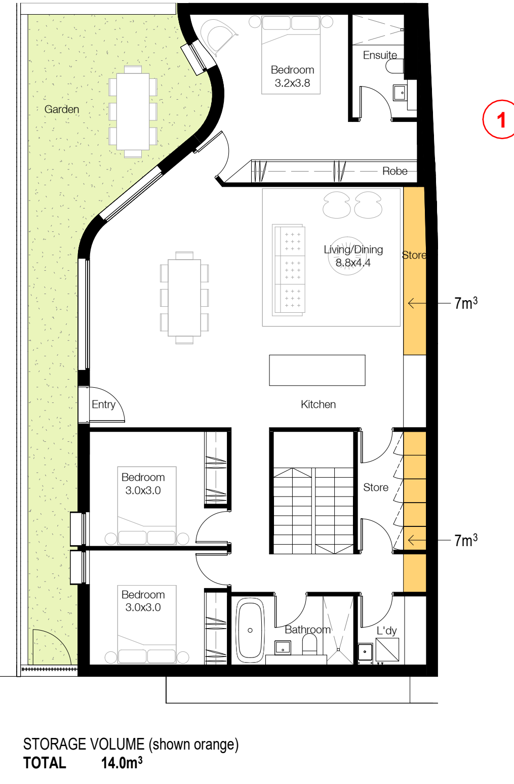
B_3 Bedroom Ground South West 1: 100@A1
