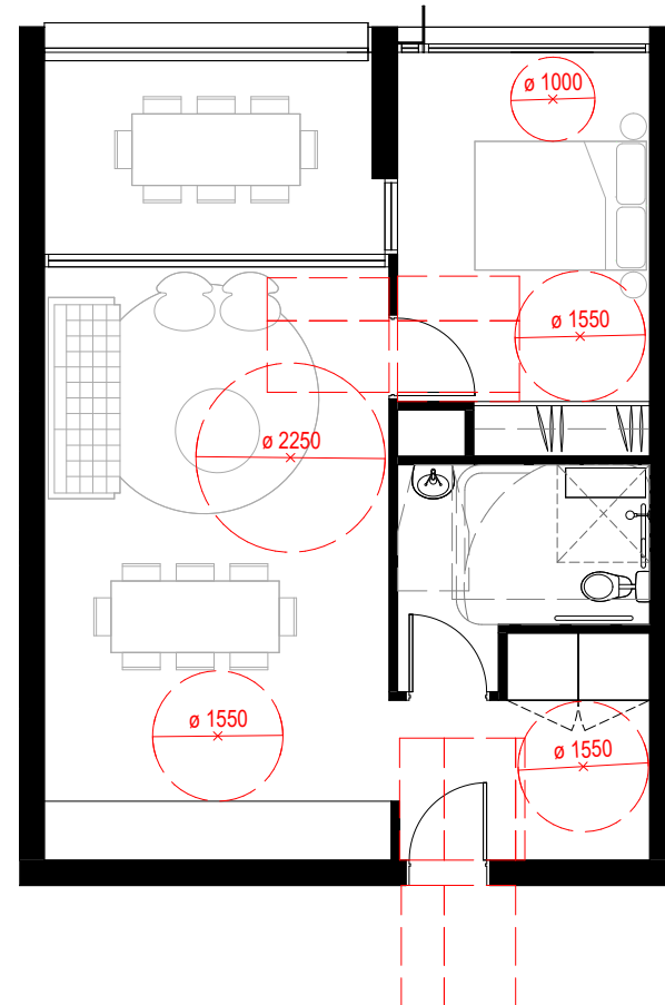
Type 3 - Post-Adapted 1 : 100@A1
