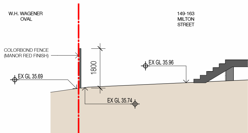
3 Building C Boundary Section 1 : 100@A1
